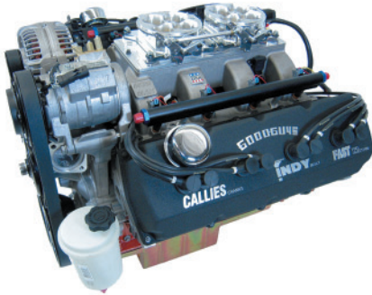
426" 6.1 HEMI
